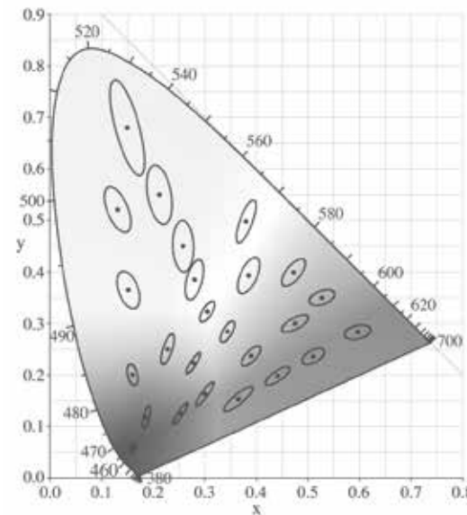
CIE 1931 (X,Y)-CHROMATICITY DIAGRAM
