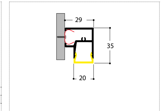
SECTION VIEW
