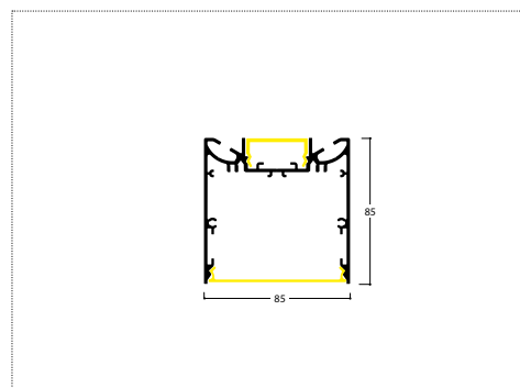
SECTION VIEW SURFACE
