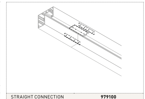
STRAIGHT CONNECTION
